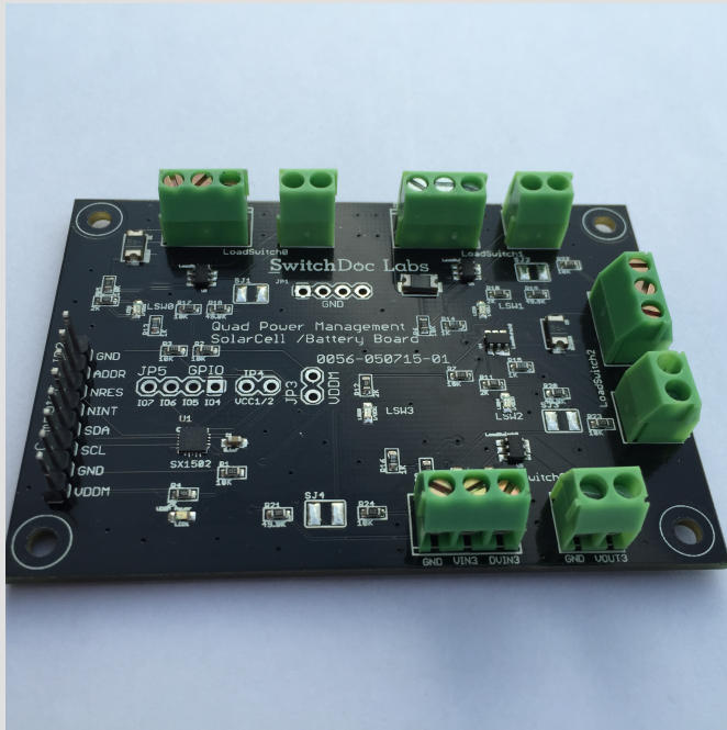
The Quad Power Management (QPM) board is an easy to use 4 channel solid state relay board controlled by I2C. Each channel can switch up to 20V and 2.33A
