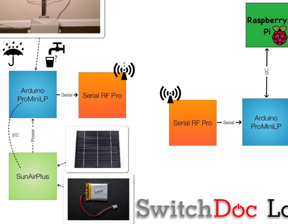
Solar WXLlink Wireless Transmit / Recieve System
